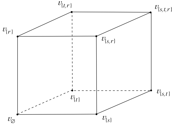
F_{\{s,t,r\}}^* viewed as a cube
