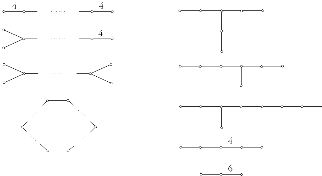
Euclidean Coxeter Groups with fundamental chamber an n -simplex, n \geq 2
