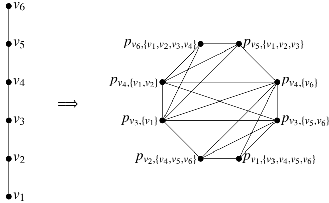
FIGURE 2. The graphs \Gamma and \tilde{\Gamma}
