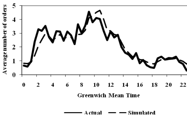
4A: Actual vs. simulated orders executed
