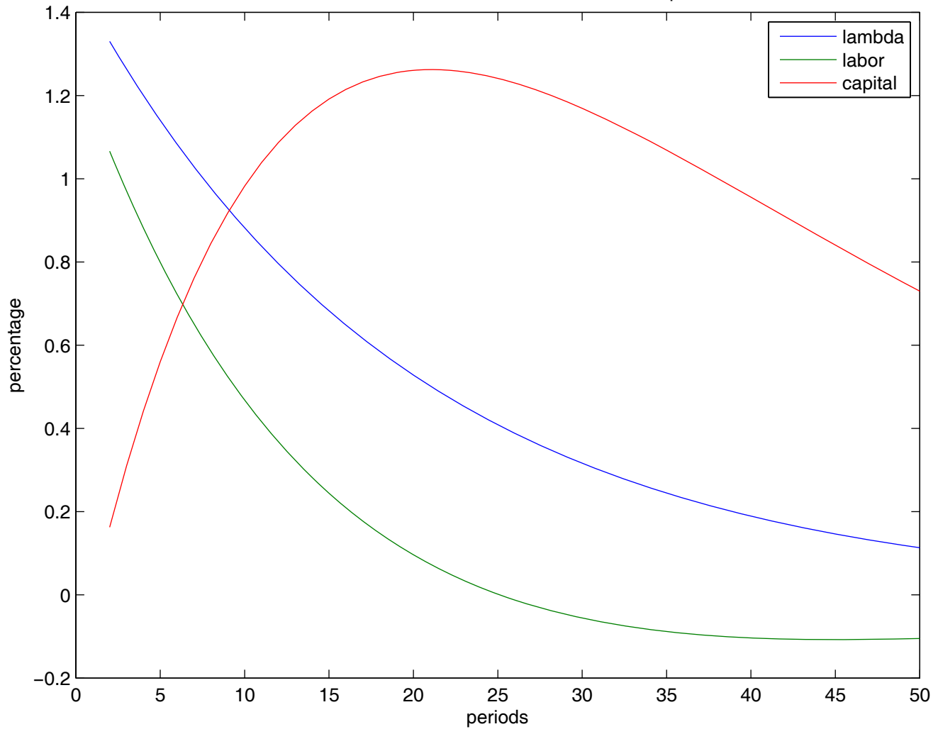
Hansen Model: Tech. Shock on labor and capital
