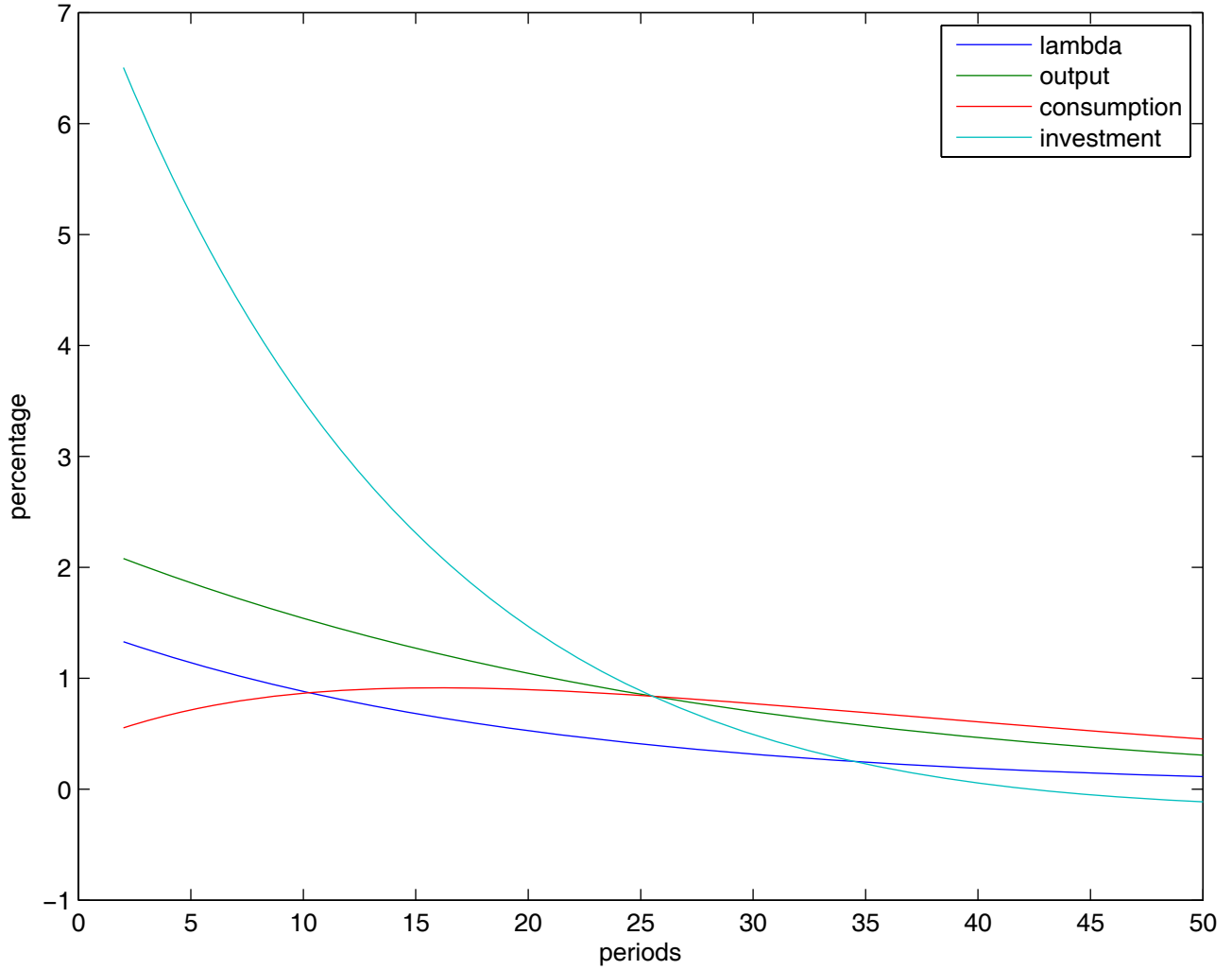
Hansen Model: Tech. Shock on q,c,i
