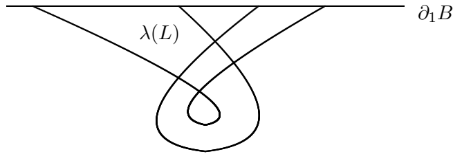
FIGURE 1. In this example, L is a square and \lambda : L \rightarrow B maps \partial_1 L = two opposite sides into \partial_1 B . The diamond shaped region is covered twice by \lambda(L) .
