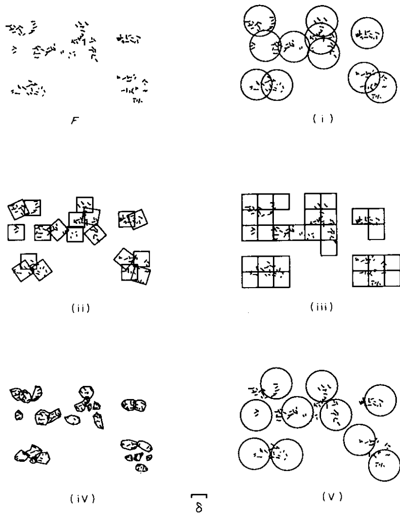
Figure 3.2 Five ways of finding the box dimension of F ; see Equivalent definitions 3.1. The number N_\delta(F) is taken to be: (i) the least number of closed balls of radius \delta that cover F ; (ii) the least number of cubes of side \delta that cover F ; (iii) the number of \delta -mesh cubes that intersect F ; (iv) the least number of sets of diameter at most \delta that cover F ; (v) the greatest number of disjoint balls of radius \delta with centres in F
