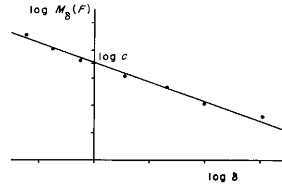
Figure 3.1 Empirical estimation of a dimension of a set F , on the power-law assumption M_\delta(F) \sim c\delta^{-s}
